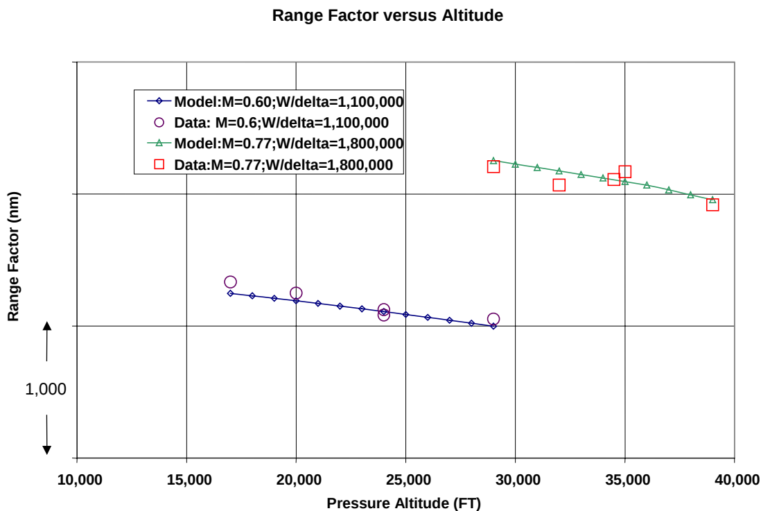
Figure 18.4 Range Factor Variation with Altitude
