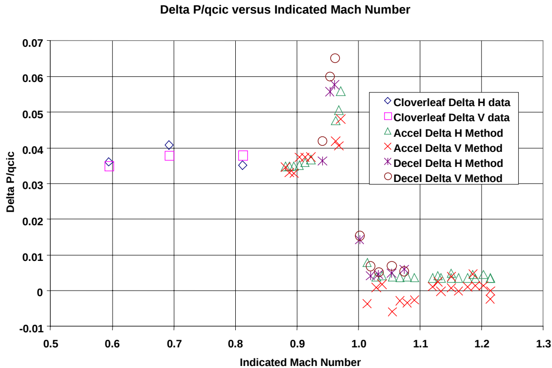
Figure 10.8 Accel-Decel Position Error Coefficient
