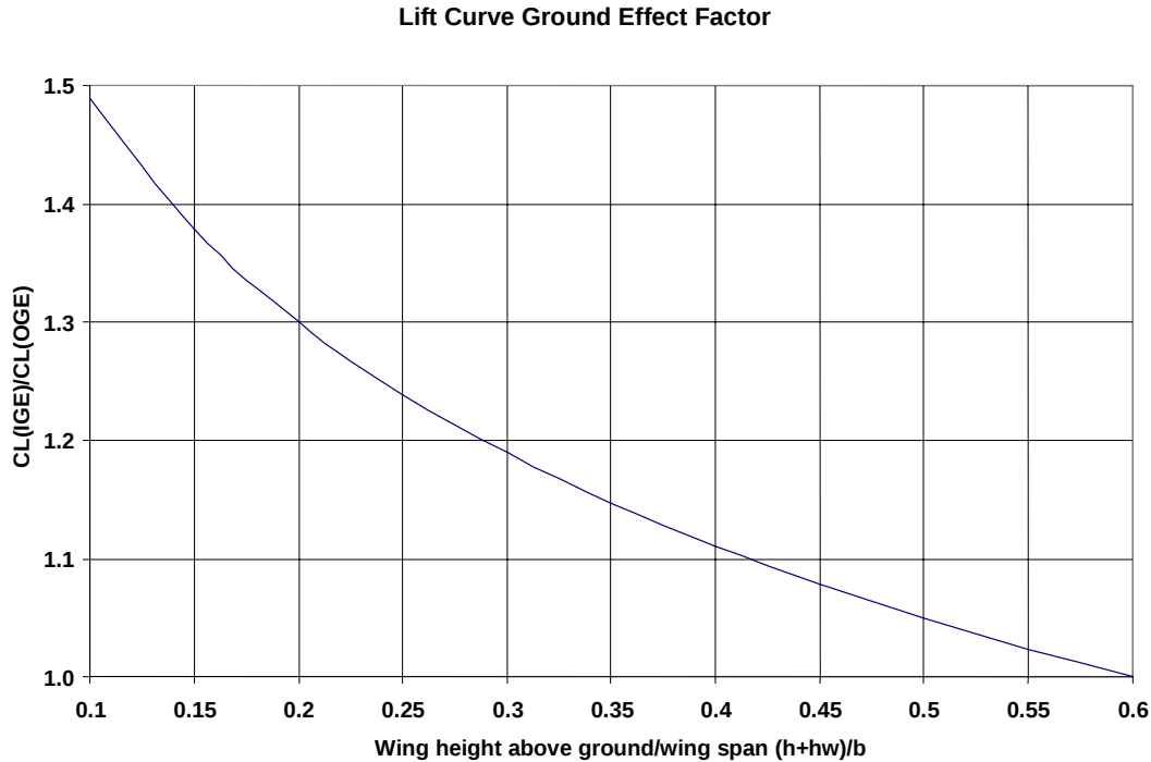
Figure 8.3 Lift Ratio In-Ground Effect
