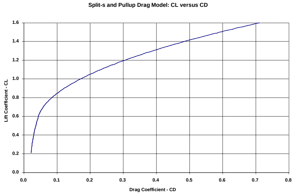
Figure 14.5 Split-S Drag Model
