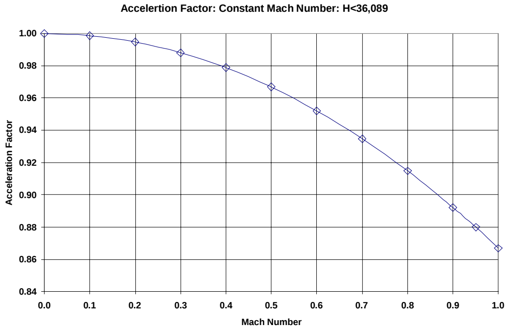
Figure 12.6 Acceleration Factor – Constant Mach Number
