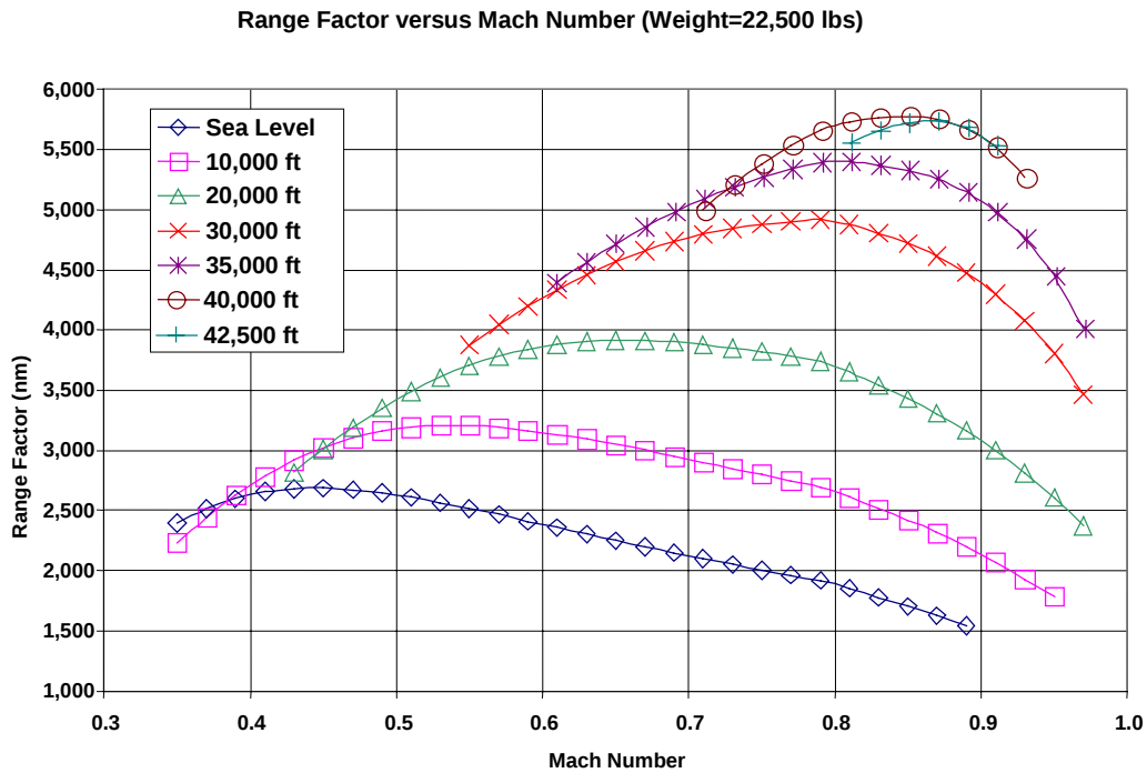
Figure 17.15 Range Factor
