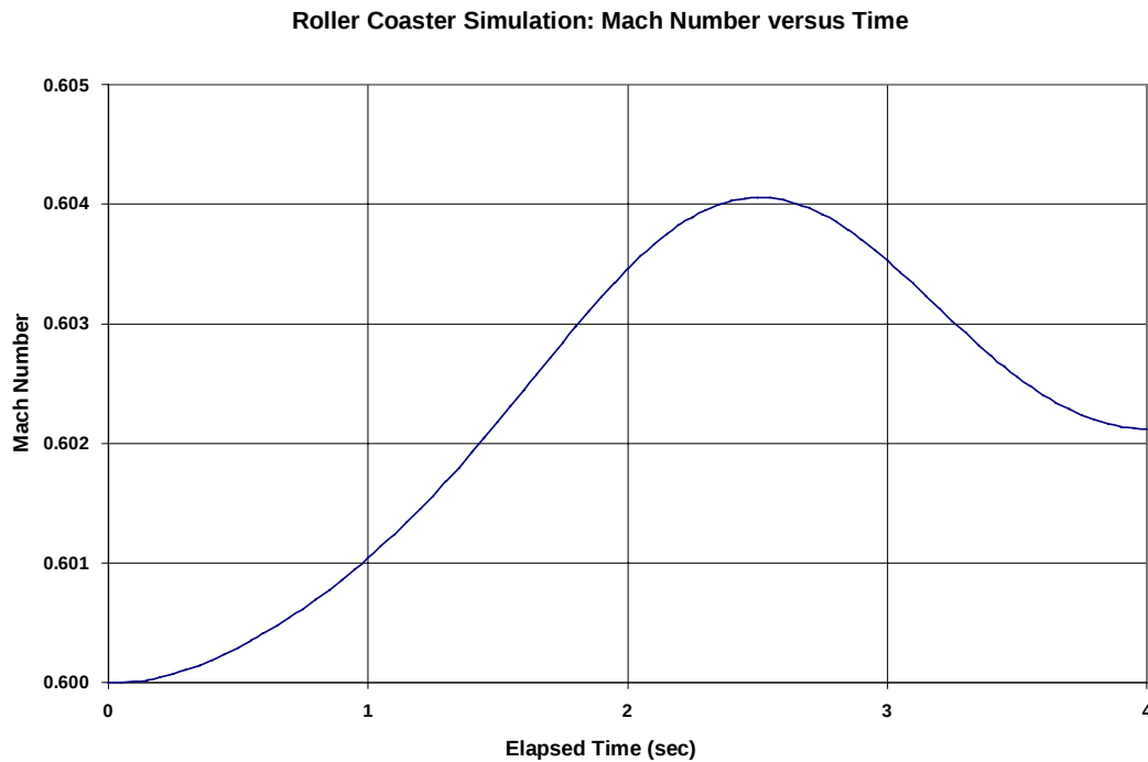
Figure 14.4 Roller Coaster Mach Number Time History
