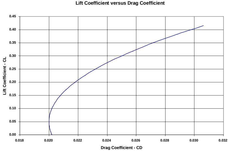
Figure 14.1 Drag Model
