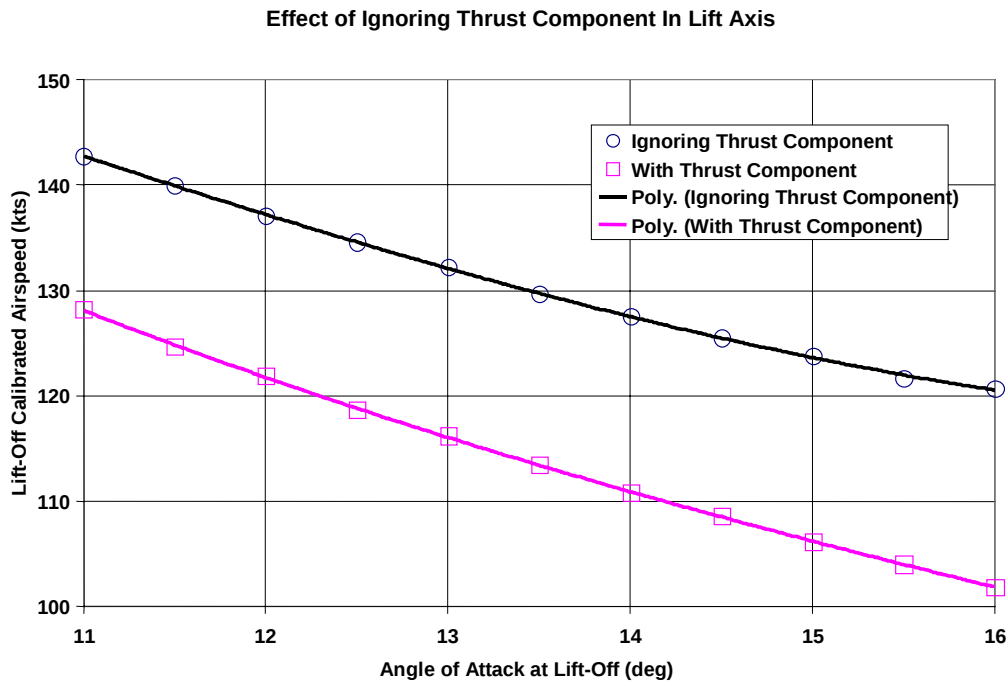
Figure 8.10 Effect of Thrust Component on Lift-Off Speed
