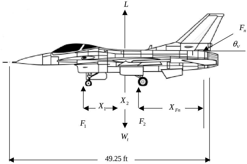
Figure 8.7 F-16 Dimensions
