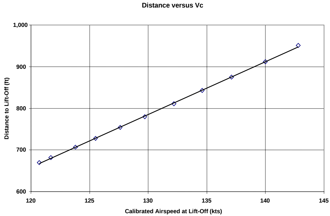
Figure 8.8 Distance to Lift-Off
