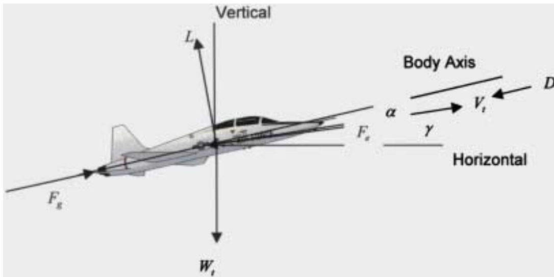
Figure 2.3 In-Flight Forces
