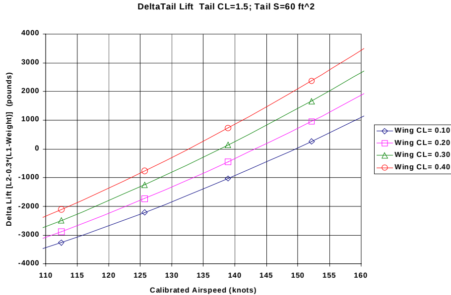
Figure 8.12 Delta Tail Lift for Tail Area = 60 ft 2
