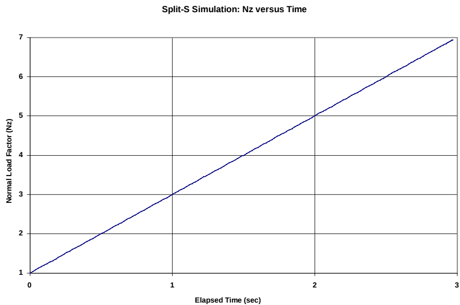
Figure 14.6 Split-S Normal Load Factor
