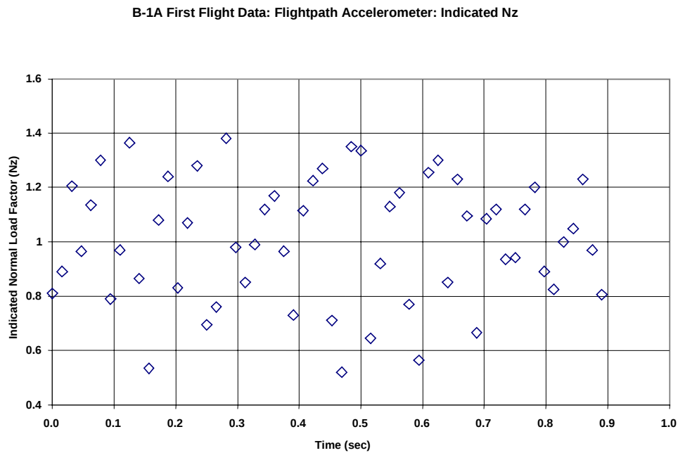
Figure 7.2 Longitudinal Load Factor – Unfiltered Data
