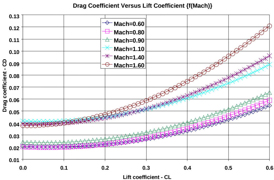
Figure 17.9 Drag Model – All Mach Numbers
