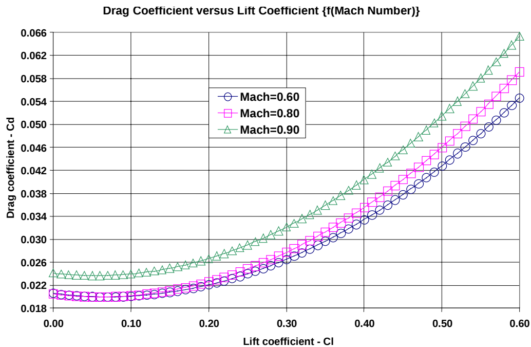
Figure 17.8 Subsonic Drag Model
