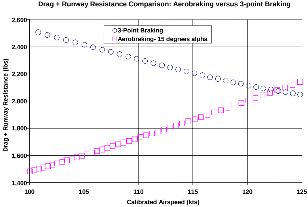
Figure 9.6 Total Resistance Force Comparison
