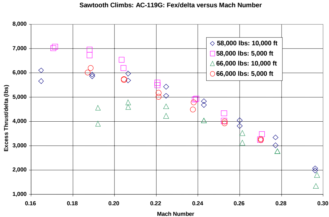
Figure 12.4 AC-119G Excess Thrust Data
