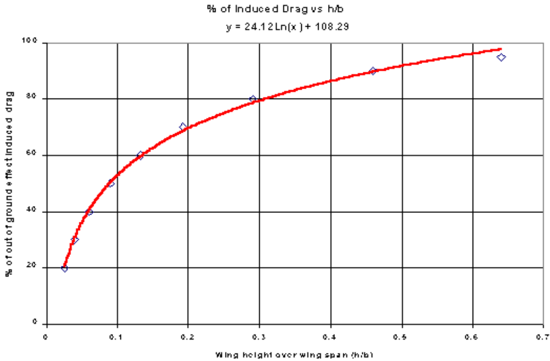
Figure 8.2 Predicted Ground Effect Drag
