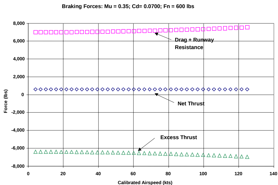
Figure 9.1 Braking Forces
