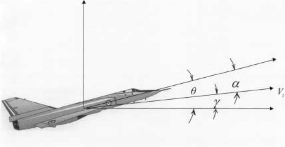
Figure 2.4 Axis System Angle Diagram
