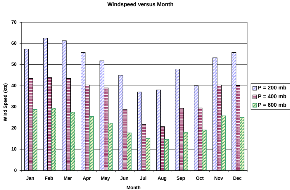
Figure A7 Windspeed
