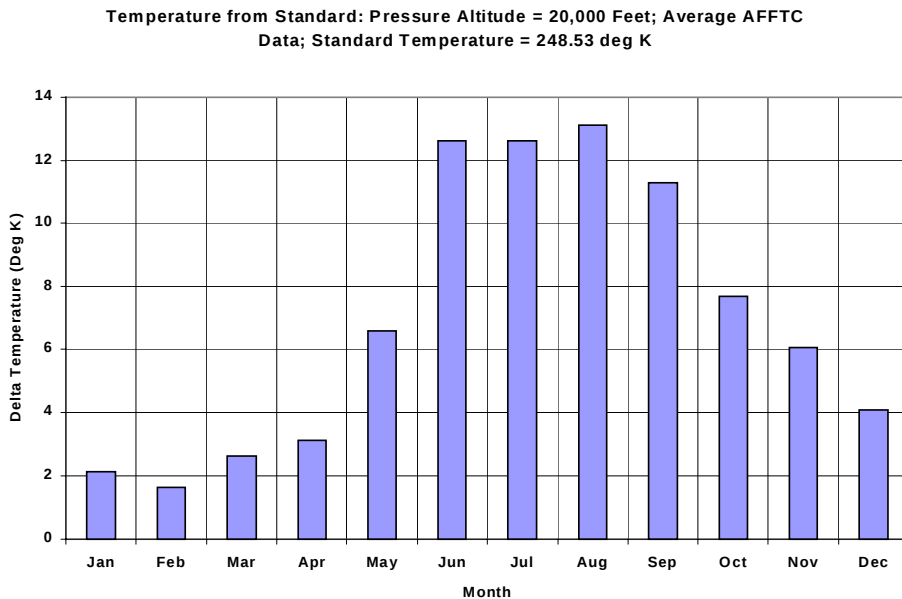
Figure A2 Delta Temperature at 20,000 Feet
