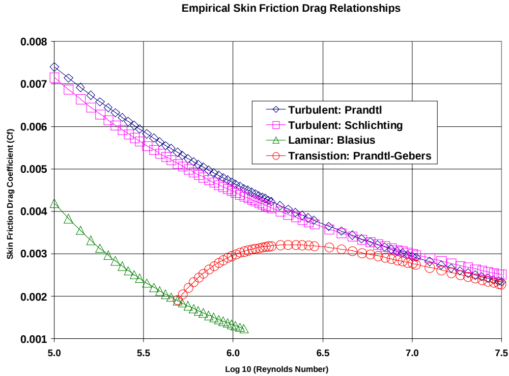
Figure 5.2 Skin Friction Drag Relationships
