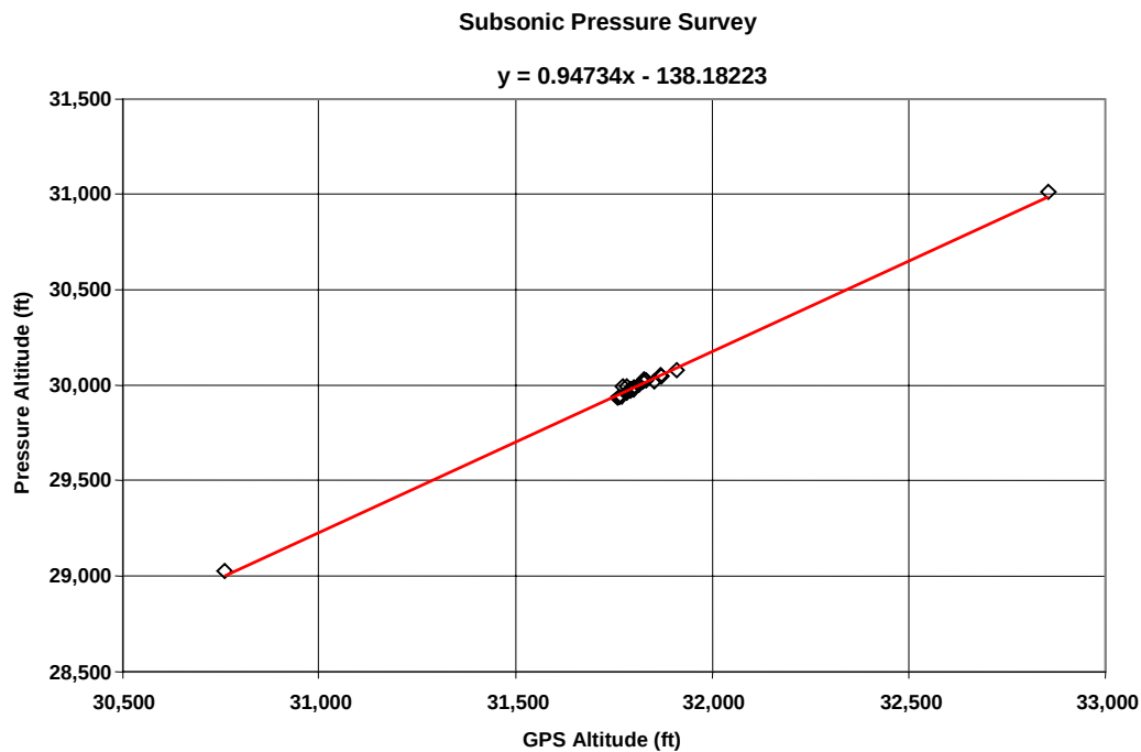
Figure 10.6 Pressure Survey
