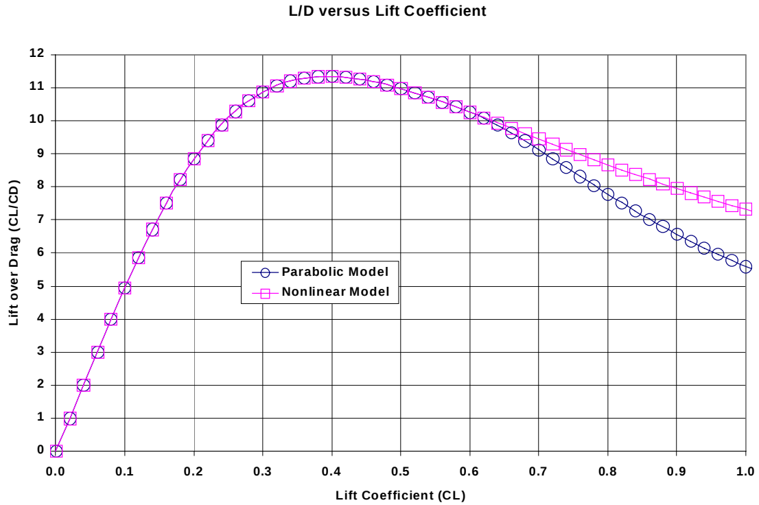
Figure 5.4 Lift-to-Drag Ratio versus Lift Coefficient
