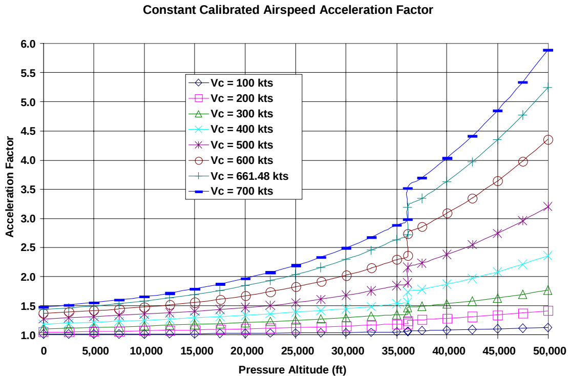
Figure 12.5 Acceleration Factor – Constant Calibrated Airspeed
