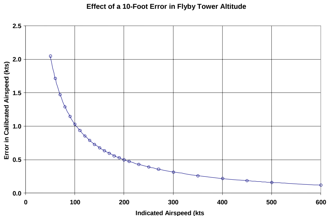
Figure 10.5 Effect of 10-Foot Error in Flyby Tower Altitude
