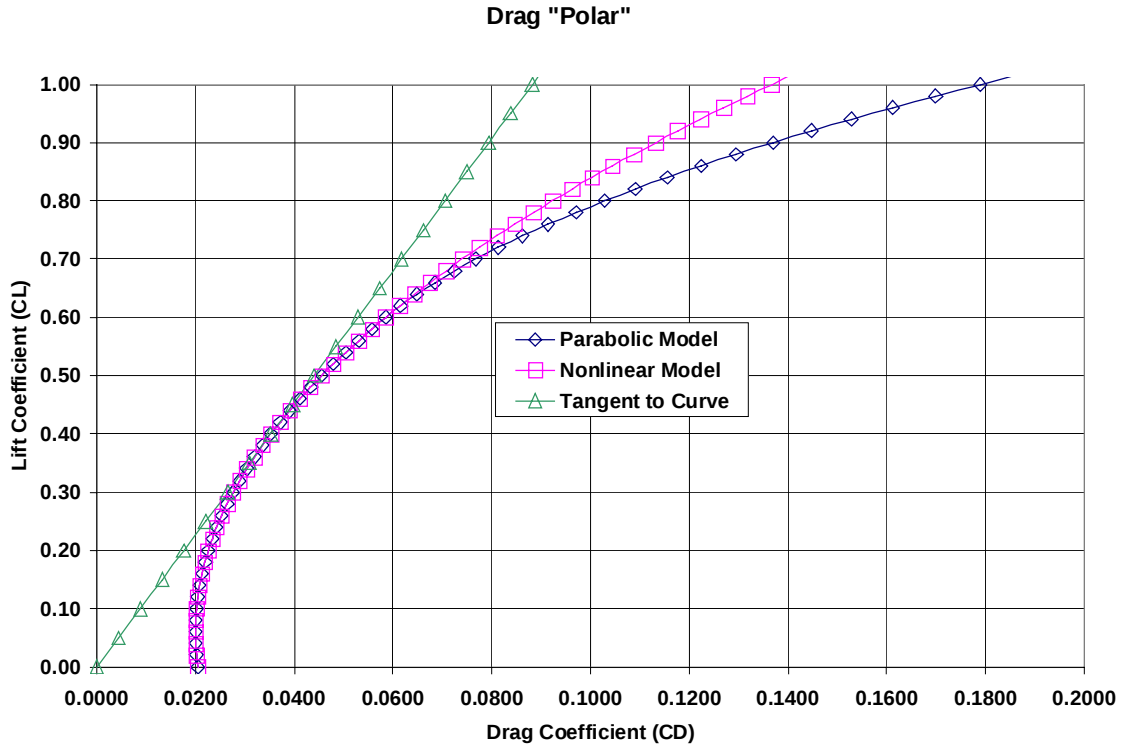
Figure 5.3 Drag Polar
