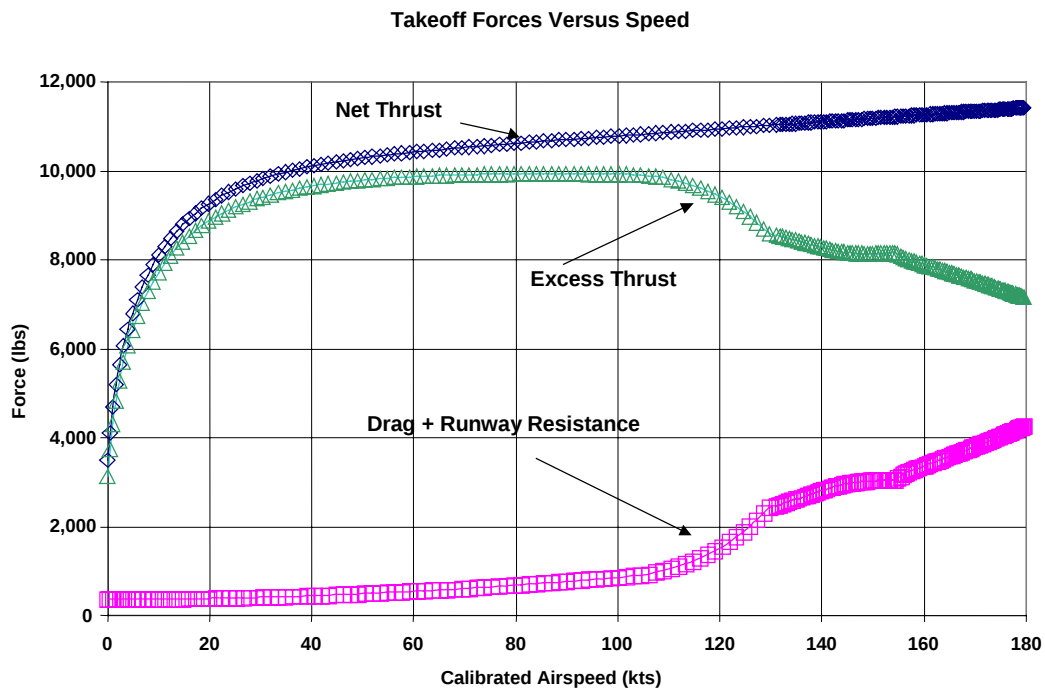
Figure 8.4 Takeoff Forces
