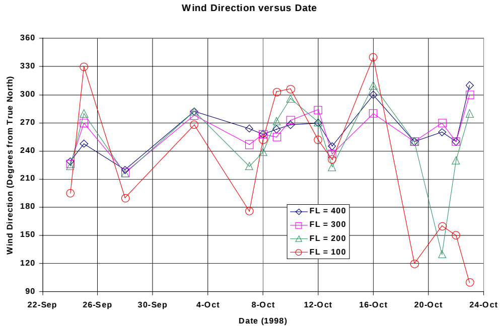
Figure B2 Wind Direction Time History
