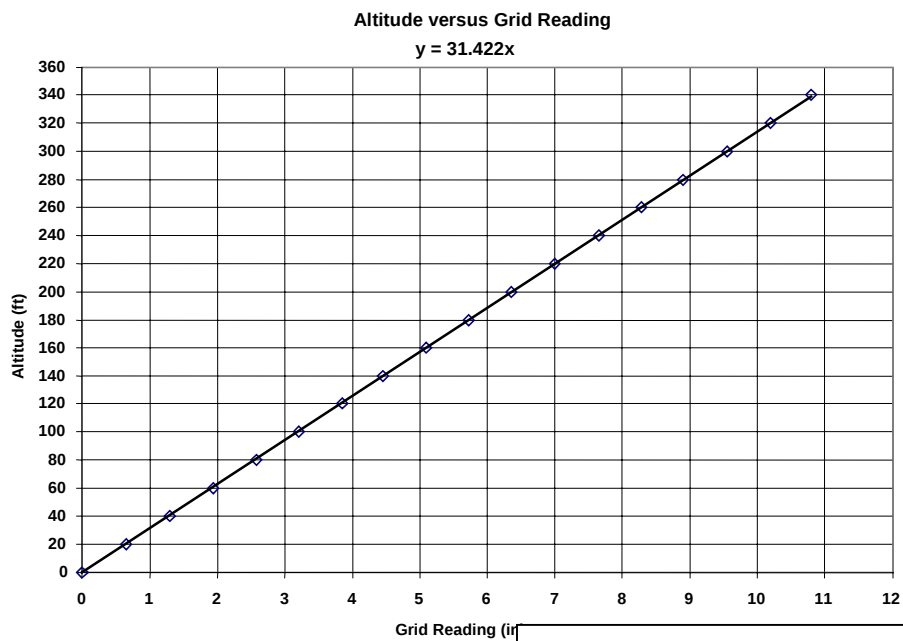
Figure 10.4 Altitude versus Grid Reading for Flyby Tower
