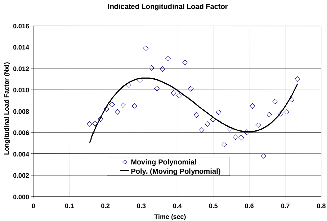
Figure 7.7 Third-Order Polynomial Fit of Filtered Longitudinal Load Factor Data
