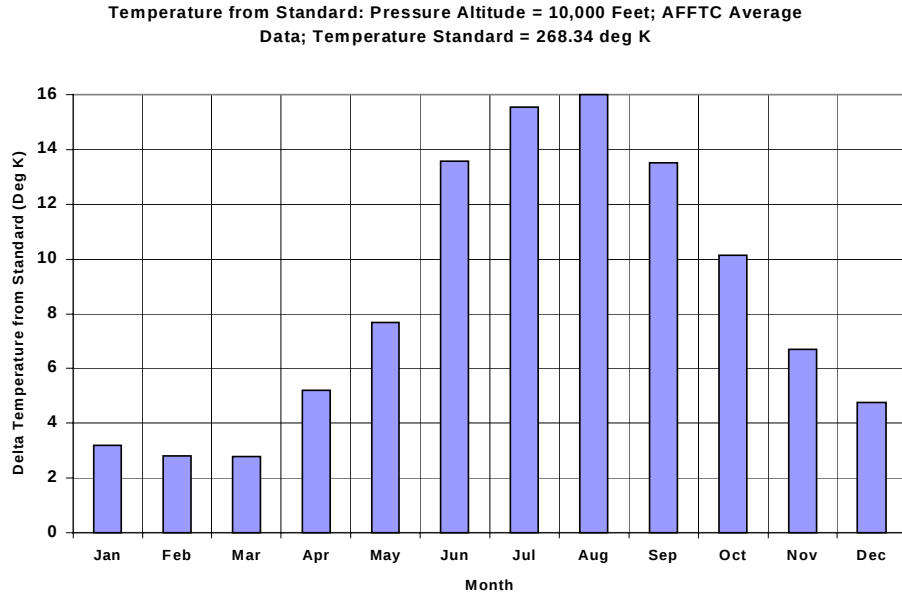
Figure A1 Delta Temperature at 10,000 Feet
