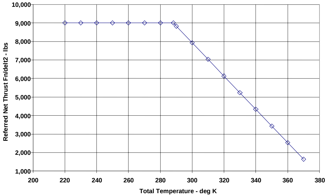
Figure 17.11 Military Referred Net Thrust
