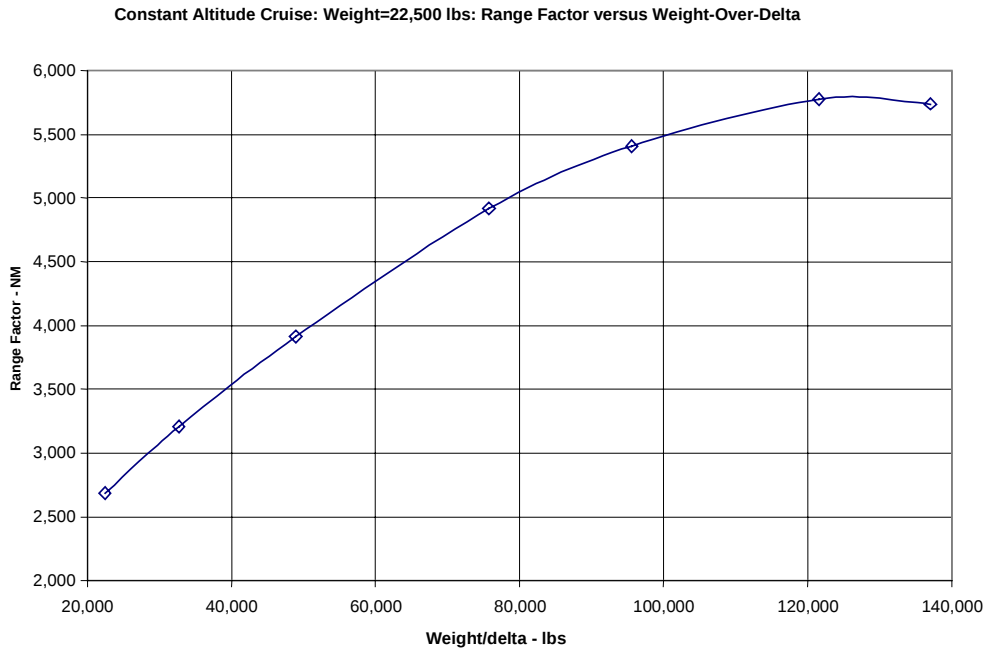
Figure 17.16 Maximum Range Factor
