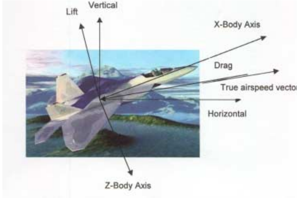
Figure 2.1 Aircraft Axis System
