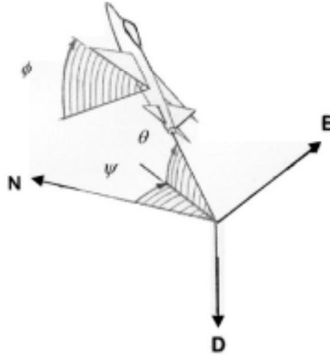
Figure 7.8 Euler Angles
