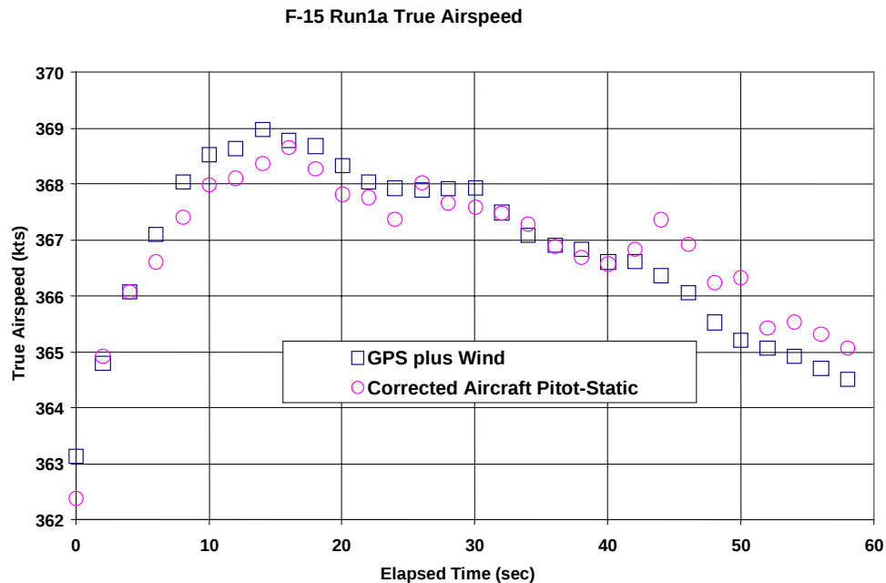
Figure 10.15 True Airspeed
