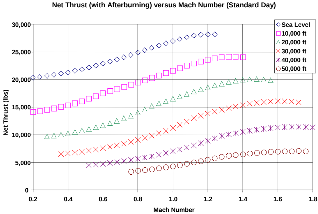
Figure 17.14 Maximum Thrust
