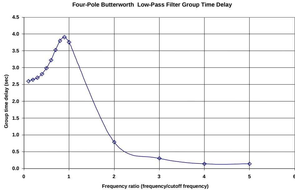
Figure 7.5 Four-Pole Butterworth Filter Group Time Delay
