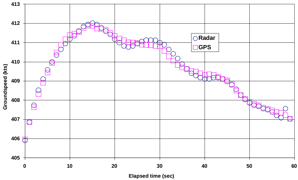
Figure 10.12 Groundspeed – Run 1a
