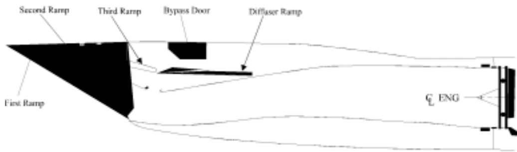
Figure 6.3 F-15 Inlet Schematic
