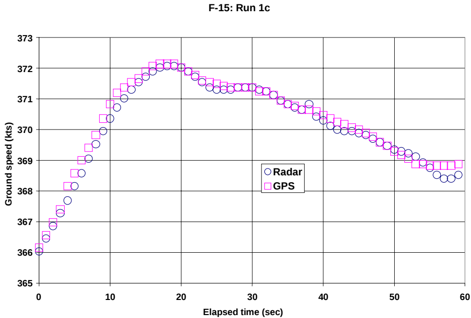
Figure 10.14 Groundspeed – Run 1c
