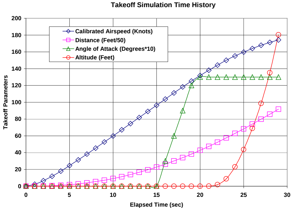
Figure 8.5 Takeoff Parameters
