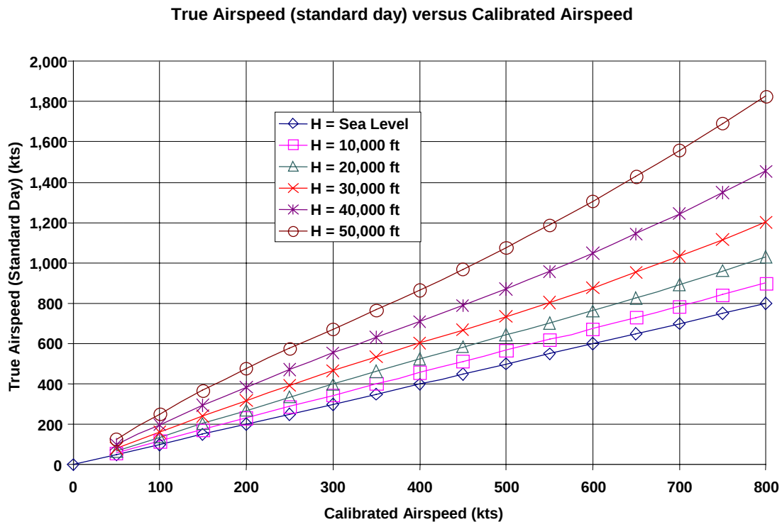
Figure 4.1 True Airspeed versus Calibrated Airspeed
