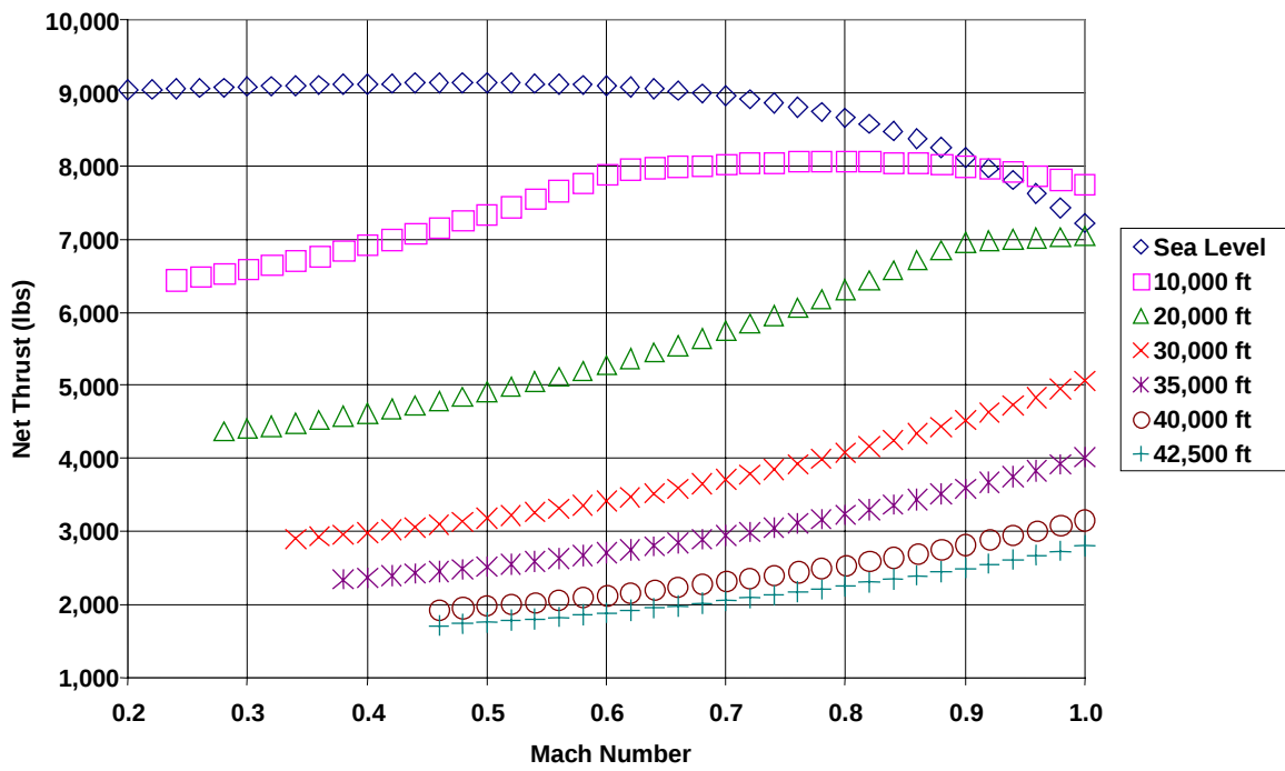
Figure 17.12 Military Thrust
