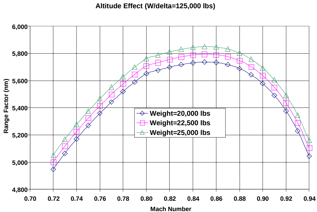
Figure 17.17 Range Factor – Altitude Effect
