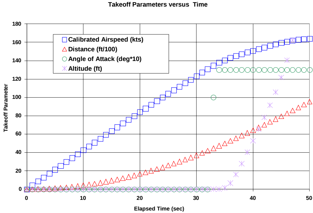
Figure 8.18 Takeoff Parameters versus Time
