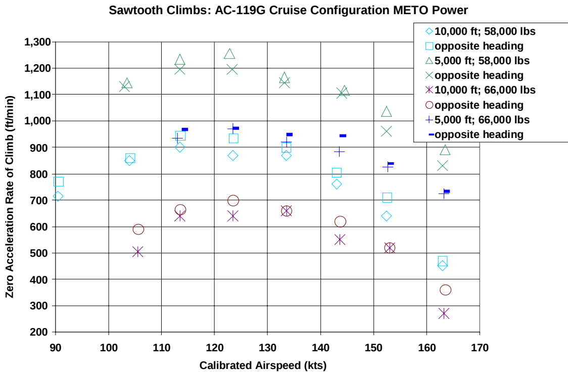
Figure 12.3 AC-119G Sawtooth Climb Data
