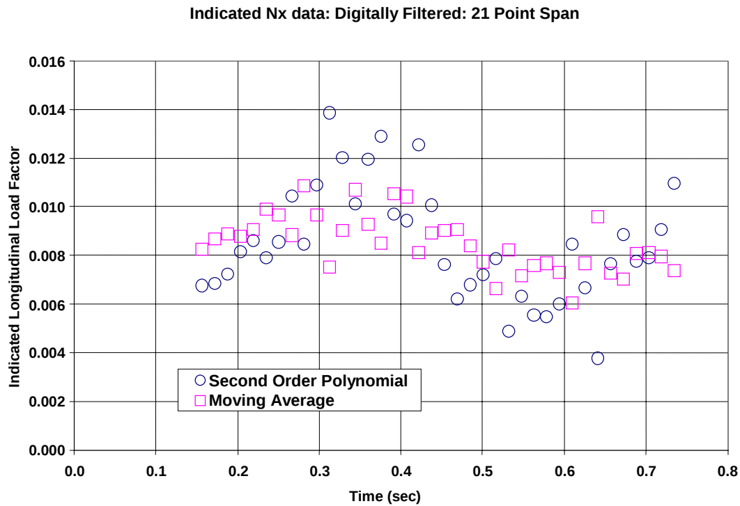
Figure 7.6 Longitudinal Load Factor – Filtered Data
