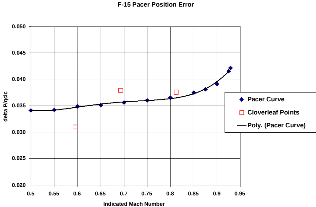
Figure 10.11 Position Error
