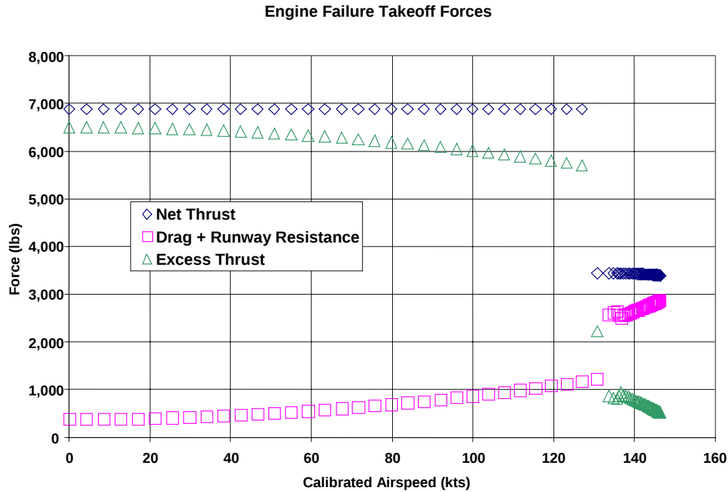
Figure 8.20 Takeoff Forces versus Airspeed: Engine Inoperative
